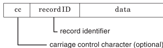
Figure 31. Record Format Line Data Record
