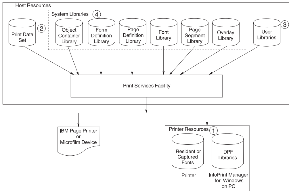
Figure 8. Resource Storage
