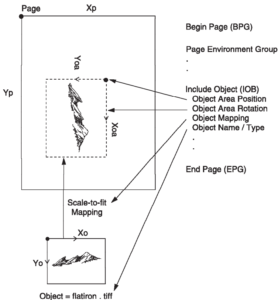
Figure 51. Use of the IOB to Include Object Container Data
